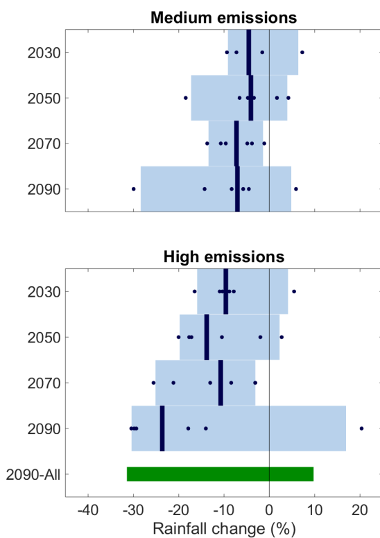
Figure 2. Projected changes (compared to 1986-2005) in annual mean rainfall for medium emissions (top) and high emissions (bottom). Bars show the 10th to 90th percentile range. Blue bars: results from the new downscaled modelling. Dark vertical line: median. Dark blue dots: individual models. Green bar: results from all available modelling (high resolution and GCM) for comparison at 2090.
