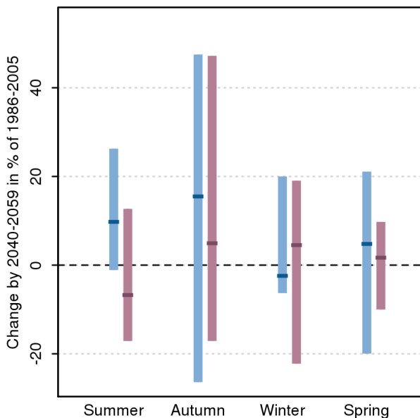
Figure 4. Projected percentage change in the 1-in-20-year daily rainfall for 2040–2059 compared to the 1986–2005. Blue bars (left): medium emissions. Purple bars (right): high emissions. Dark horizontal lines: median.
