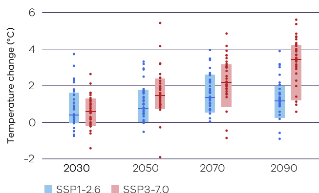
Figure 3. Projected changes in the temperature of very hot days (99.9th percentile) over the Central Highlands for low emissions (blue) and high emissions (red) relative to a 1986–2005 baseline, for four future time periods. Data sourced from Australia-wide and NARClIM2.0 ~4 km climate modelling. See guidance on interpreting this figure at the back of the report.
