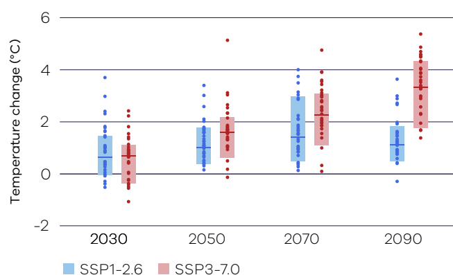
Figure 3. Projected changes in the temperature of very hot days (99.9th percentile) over the Loddon Campaspe region for low emissions (blue) and high emissions (red) relative to a 1986–2005 baseline, for four future time periods. Data sourced from Australia-wide and NARClIM2.0 ~4 km climate modelling. See guidance on interpreting this figure at the back of the report.
