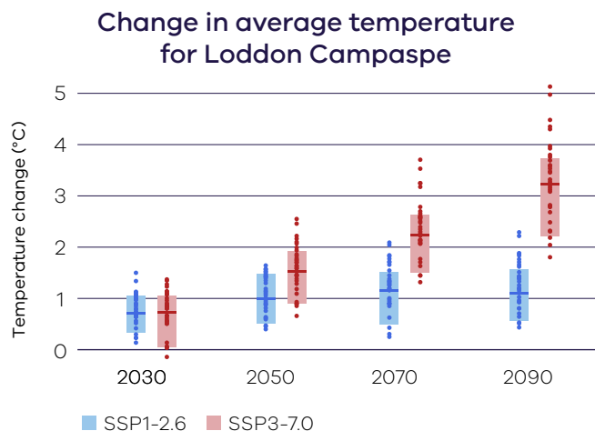
Figure 2. Projected changes in annual mean temperature over the Loddon Campaspe region, for low emissions (blue) and high emissions (red) relative to a 1986–2005 baseline, for four future time periods. Data sourced from Australia-wide and NARClIM2.0 ~4 km climate modelling. See guidance on interpreting this figure at the back of the report.
