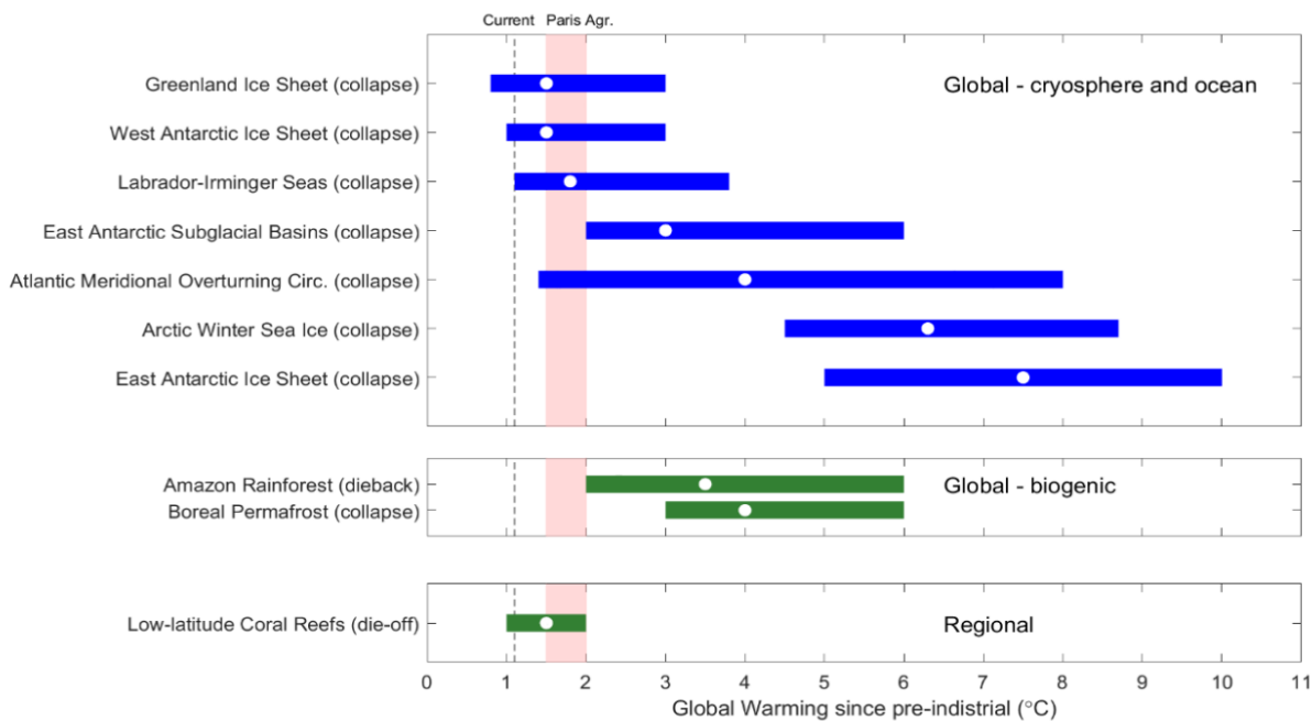
Figure 1. Nine global climate tipping points and one relevant regional tipping point listed in a recent global review. Horizontal bars show the review’s assessed ranges of global warming where the tipping may be triggered. Assessed ranges may differ from other studies. Source: CSIRO, 2024 (adapted from Armstrong McKay et al., 2022)
