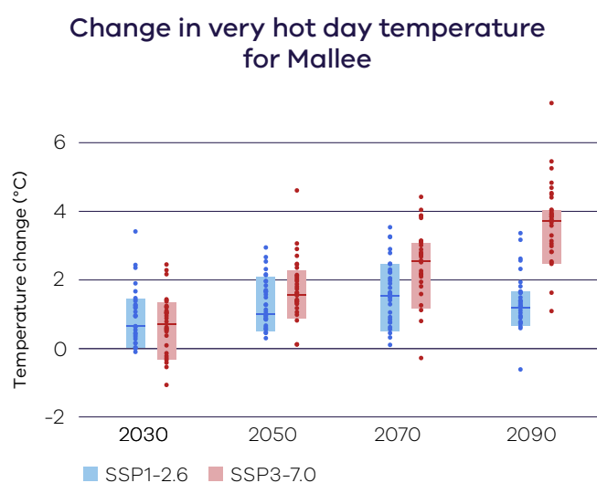
Figure 3. Projected changes in the temperature of very hot days (99.9th percentile) over the Mallee for low emissions (blue) and high emissions (red) relative to a 1986–2005 baseline, for four future time periods. Data sourced from Australia-wide and NARClIM2.0 ~4 km climate modelling. See guidance on interpreting this figure at the back of the report.
