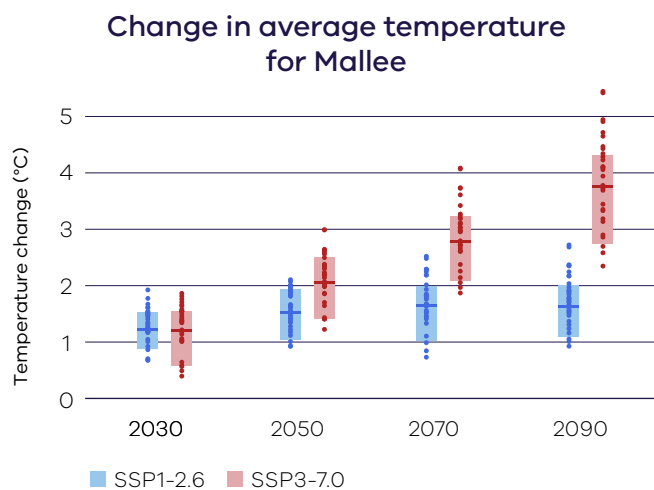
Figure 2. Projected changes in annual mean temperature over the Mallee region, for low emissions (blue) and high emissions (red) relative to a 1986–2005 baseline, for four future time periods. Data sourced from Australia-wide and NARClIM2.0 ~4 km climate modelling. See guidance on interpreting this figure at the back of the report.
