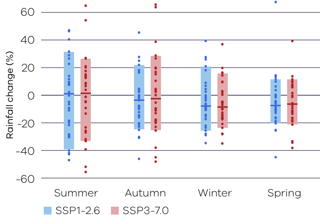
Figure 5. Projected changes in seasonal rainfall for the Mallee region for 2050 (2040–2059) for low (blue) and high (red) emissions scenarios, relative to a 1986–2005 baseline. Data sourced from Australia-wide and NARClIM2.0 ~4 km climate modelling. See guidance on interpreting this figure at the back of the report.
