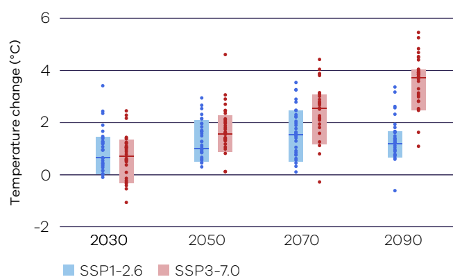
Figure 3. Projected changes in the temperature of very hot days (99.9th percentile) over the Mallee for low emissions (blue) and high emissions (red) relative to a 1986–2005 baseline, for four future time periods. Data sourced from Australia-wide and NARClIM2.0 ~4 km climate modelling. See guidance on interpreting this figure at the back of the report.
