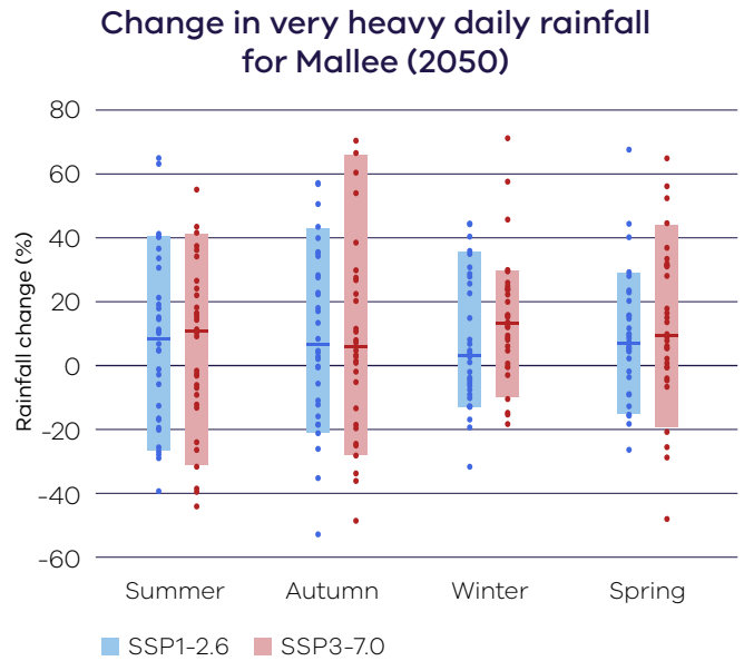
Figure 6. Projected changes on very heavy rainfall days (99.9th percentile) for the Mallee, by season for 2050 (2040–2059) under low (blue) and high (red) emissions scenarios, relative to a 1986–2005 baseline. Data sourced from Australia-wide and NARClIM2.0 ~4 km climate modelling. See guidance on interpreting this figure at the back of the report.
