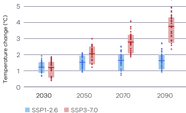
Figure 2. Projected changes in annual mean temperature over the Mallee region, for low emissions (blue) and high emissions (red) relative to a 1986–2005 baseline, for four future time periods. Data sourced from Australia-wide and NARClIM2.0 ~4 km climate modelling. See guidance on interpreting this figure at the back of the report.
