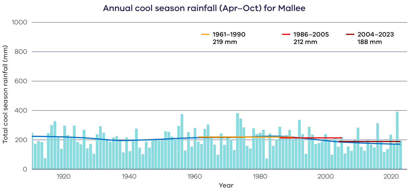
Figure 4. Observed cool season rainfall for the Mallee region from 1910–2023. The blue line shows the long-term trend. Average rainfall is also shown for a number of time periods: the BOMs 1961–1990 baseline, the 1986–2005 baseline used for the projections in this report and the most recent 20 years 2004–2023. Data sourced from the Australian Gridded Climate Dataset (AGCD).
