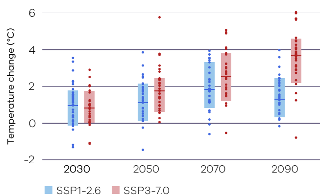
Figure 3. Projected changes in the temperature of very hot days (99.9th percentile) over the Ovens Murray region for low emissions (blue) and high emissions (red) relative to a 1986–2005 baseline, for four future time periods. Data sourced from Australia-wide and NARcliM2.0 ~4 km climate modelling. See guidance on interpreting this figure at the back of the report.
