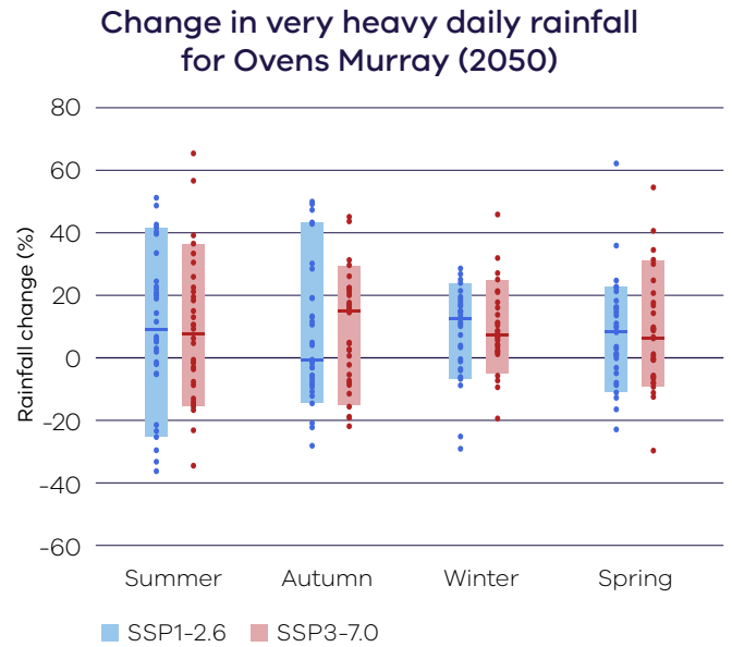
Figure 6. Projected changes on very heavy rainfall days (99.9th percentile) for the Ovens Murray region, by season for 2050 (2040–2059) under low (blue) and high (red) emissions scenarios, relative to a 1986–2005 baseline. Data sourced from Australia-wide and NARClm2.0 ~4 km climate modelling. See guidance on interpreting this figure at the back of the report.
