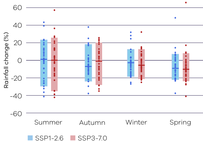
Figure 5. Projected changes in seasonal rainfall for the Ovens Murray region for 2050 (2040–2059) for low (blue) and high (red) emissions scenarios, relative to a 1986–2005 baseline. Data sourced from Australia-wide and NARClIM2.0 ~4 km climate modelling. See guidance on interpreting this figure at the back of the report.
