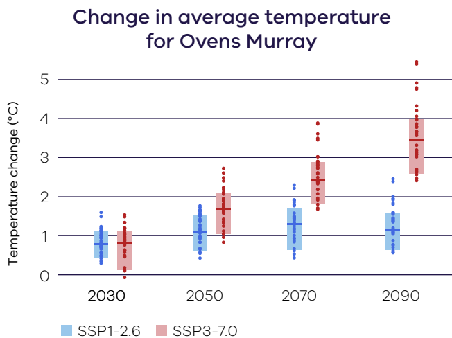
Figure 2. Projected changes in annual mean temperature over the Ovens Murray region, for low emissions (blue) and high emissions (red) relative to a 1986–2005 baseline, for four future time periods. Data sourced from Australia-wide and NARClIM2.0 ~4 km climate modelling. See guidance on interpreting this figure at the back of the report.
