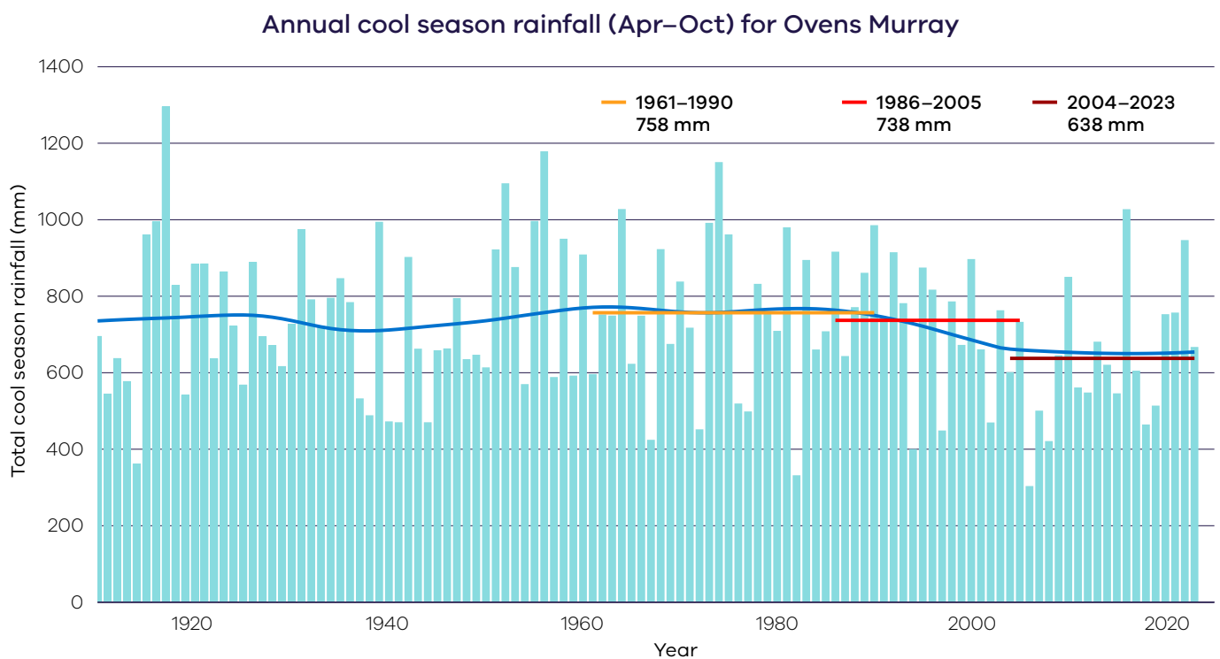
Figure 4. Observed cool season rainfall for the Ovens Murray region from 1910–2023. The blue line shows the long-term trend. Average rainfall is also shown for a number of time periods: the BOMs 1961–1990 baseline, the 1986–2005 baseline used for the projections in this report and the most recent 20 years 2004–2023. Data sourced from the Australian Gridded Climate Dataset (AGCD).
