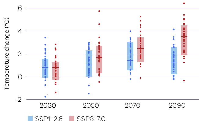
Figure 3. Projected changes in the temperature of very hot days (99.9th percentile) over Gippsland for low emissions (blue) and high emissions (red) relative to a 1986–2005 baseline, for four future time periods. Data sourced from Australia-wide and NARClIM2.0 ~4 km climate modelling. See guidance on interpreting this figure at the back of the report.
