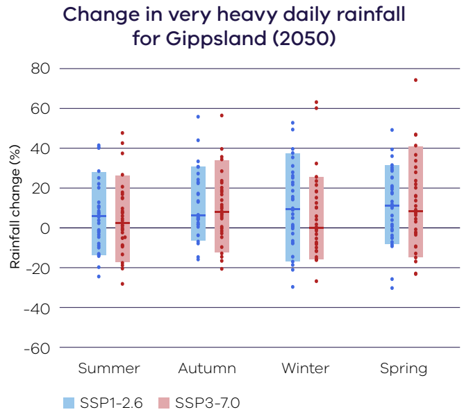
Figure 6. Projected changes on very heavy rainfall days (99.9th percentile) for Gippsland, by season for 2050 (2040–2059) under low (blue) and high (red) emissions scenarios, relative to a 1986–2005 baseline. Data sourced from Australia-wide and NARClIM2.0 ~4 km climate modelling. See guidance on interpreting this figure at the back of the report.
