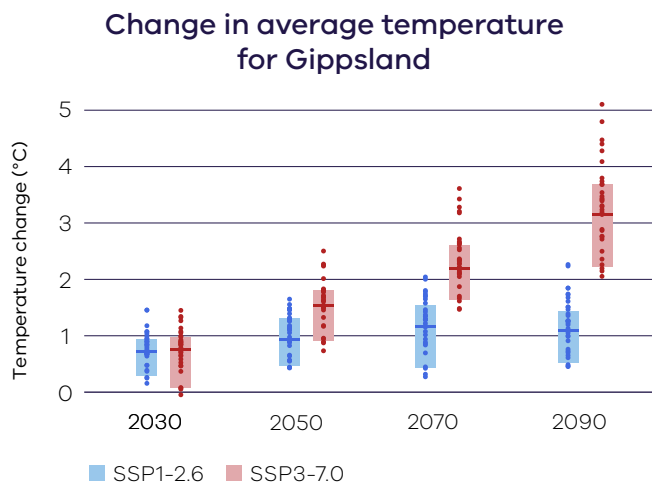
Figure 2. Projected changes in annual mean temperature over the Gippsland region, for low emissions (blue) and high emissions (red) relative to a 1986–2005 baseline, for four future time periods. Data sourced from Australia-wide and NARClIM2.0 ~4 km climate modelling. See guidance on interpreting this figure at the back of the report.
