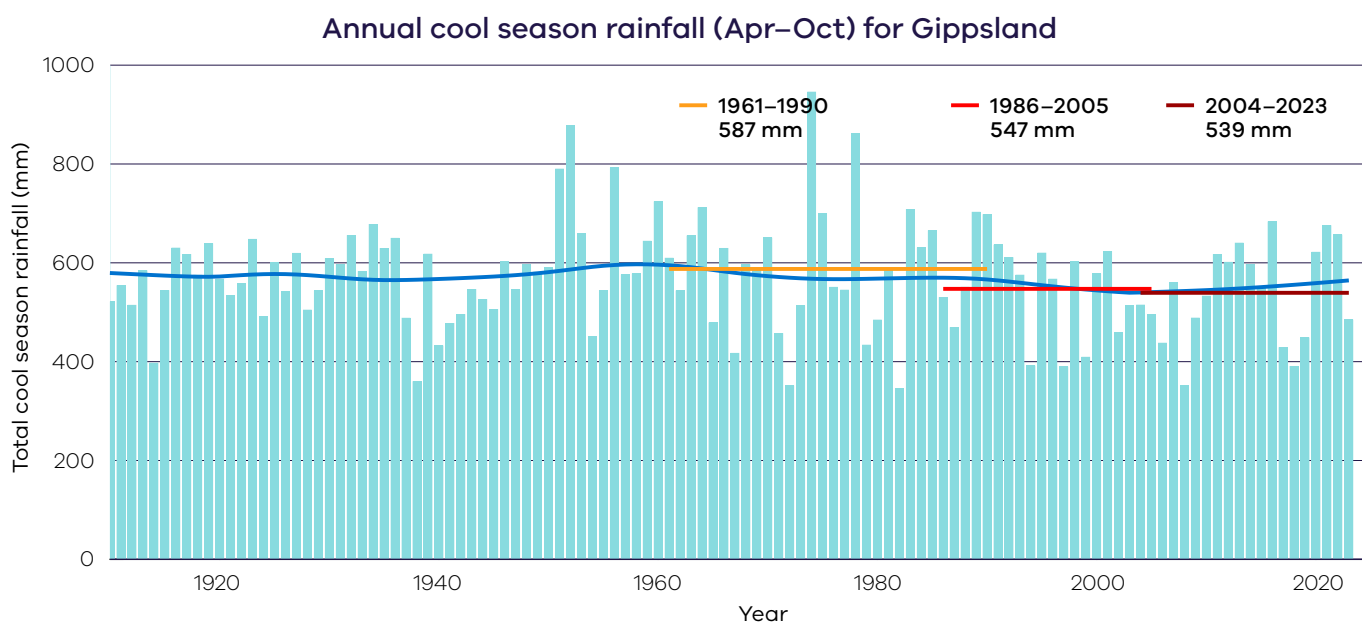
Figure 4. Observed cool season rainfall for Gippsland from 1910–2023. The blue line shows the long-term trend. Average rainfall is also shown for a number of time periods: the BOMs 1961–1990 baseline, the 1986–2005 baseline used for the projections in this report and the most recent 20 years 2004–2023. Data sourced from the Australian Gridded Climate Dataset (AGCD).
