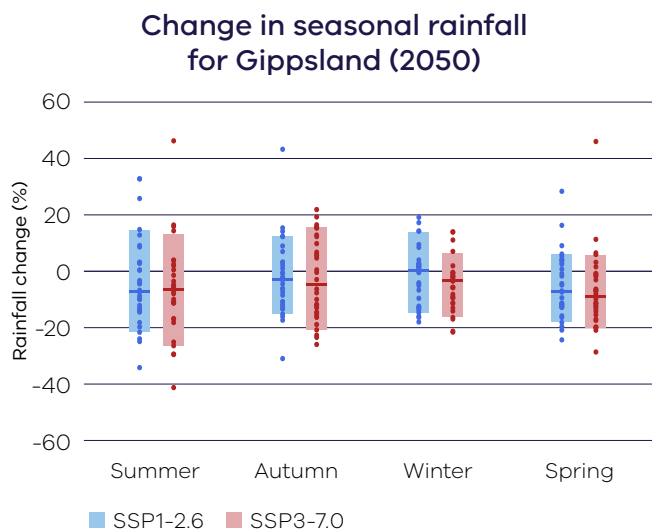
Figure 5. Projected changes in seasonal rainfall for Gippsland for 2050 (2040–2059) for low (blue) and high (red) emissions scenarios, relative to a 1986–2005 baseline. Data sourced from Australia-wide and NARClIM2.0 ~4 km climate modelling. See guidance on interpreting this figure at the back of the report.
