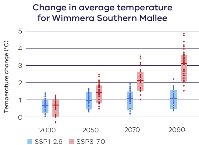
Figure 2. Projected changes in annual mean temperature over the Wimmera Southern Mallee region, for low emissions (blue) and high emissions (red) relative to a 1986–2005 baseline, for four future time periods. Data sourced from Australia-wide and NARClIM2.0 ~4 km climate modelling. See guidance on interpreting this figure at the back of the report.
