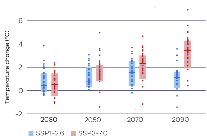
Figure 3. Projected changes in the temperature of very hot days 4 (99.9th percentile) over the Wimmera Southern Mallee region for low emissions (blue) and high emissions (red) relative to a 1986–2005 baseline, for four future time periods. Data sourced from Australia-wide and NARClIM2.0 ~4 km climate modelling. See guidance on interpreting this figure at the back of the report.
