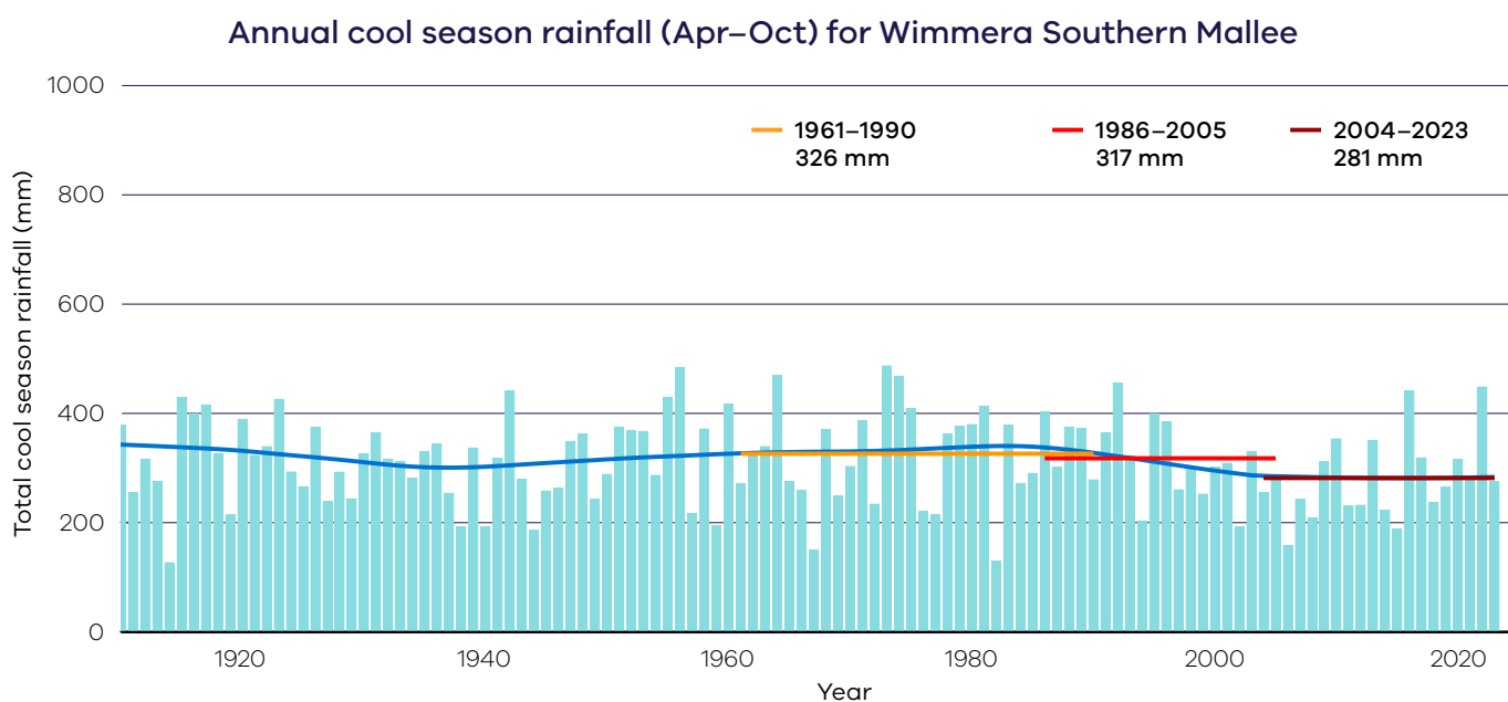
Figure 4. Observed cool season rainfall for the Wimmera Southern Mallee region from 1910–2023. The blue line shows the long-term trend. Average rainfall is also shown for a number of time periods: the BOMs 1961–1990 baseline, the 1986–2005 baseline used for the projections in this report and the most recent 20 years 2004–2023. Data sourced from the Australian Gridded Climate Dataset (AGCD).
