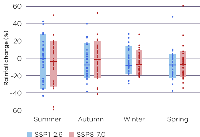
Figure 5. Projected changes in seasonal rainfall for the Wimmera Southern Mallee region for 2050 (2040–2059) for low (blue) and high (red) emissions scenarios, relative to a 1986–2005 baseline. Data sourced from Australia-wide and NARClIM2.0 ~4 km climate modelling. See guidance on interpreting this figure at the back of the report.
