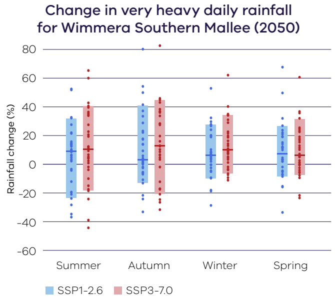
Figure 6. Projected changes on very heavy rainfall days (99.9th percentile) for the Wimmera Southern Mallee region, by season for 2050 (2040–2059) under low (blue) and high (red) emissions scenarios, relative to a 1986–2005 baseline. Data sourced from Australia-wide and NARCIIM2.0 ~4 km climate modelling. See guidance on interpreting this figure at the back of the report.
