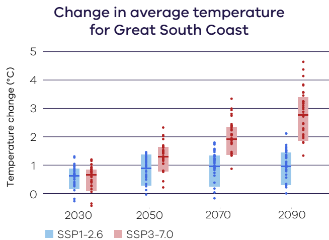
Figure 2. Projected changes in annual mean temperature over the Great South Coast region, for low emissions (blue) and high emissions (red) relative to a 1986–2005 baseline, for four future time periods. Data sourced from Australia-wide and NARClIM2.0 ~4 km climate modelling. See guidance on interpreting this figure at the back of the report.
