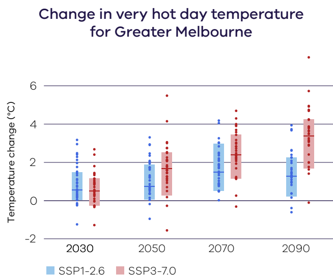
Figure 3. Projected changes in the temperature of very hot days (99.9th percentile) over Greater Melbourne for low emissions (blue) and high emissions (red) relative to a 1986–2005 baseline, for four future time periods.
