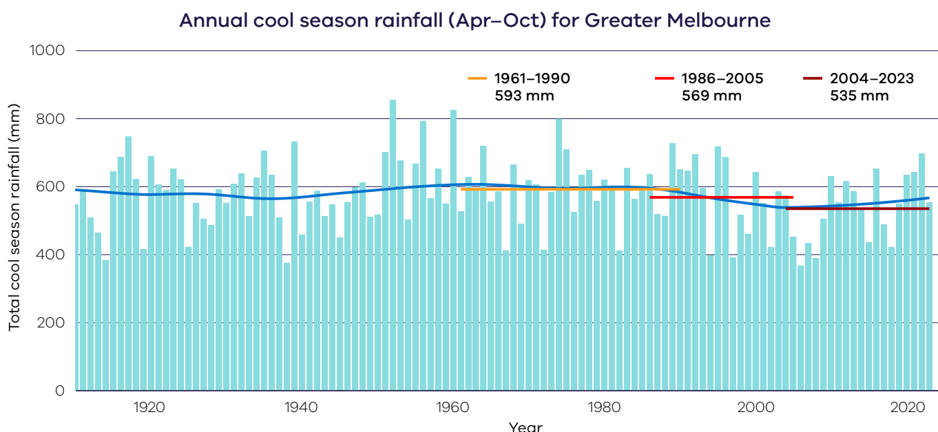
Figure 4. Observed cool season rainfall for Greater Melbourne from 1910–2023. The blue line shows the long-term trend. Average rainfall is also shown for a number of time periods: the BOMs 1961–1990 baseline, the 1986–2005 baseline used for the projections in this report and the most recent 20 years 2004–2023. Data sourced from the Australian Gridded Climate Dataset (AGCD).
